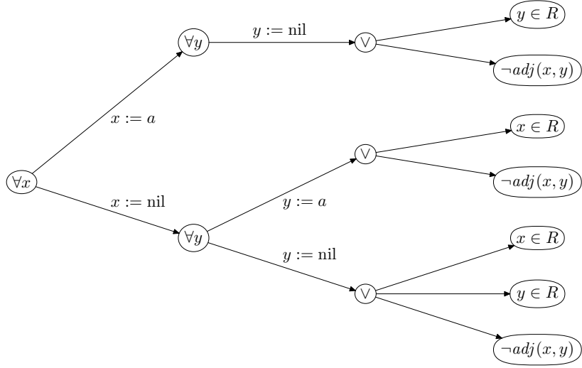
Figure 3: Simplified schematic of \text{reduce}(\mathcal{A}, X, vc) , where \mathcal{A} has universe A = \{a\} , X = A and a \notin R^{\mathcal{A}} . If any of the symbols x or y remains uninterpreted (cases x := \text{nil} and y := \text{nil} in the figure), then some of the plays in \mathcal{EMC}(\mathcal{A}, \emptyset, vc) end with a draw and still persist in the reduced game. If \mathcal{A} = \mathcal{A}_i and X = X_i for a node i of a tree decomposition, then this essentially means that it is still open whether nodes in the “future” of i will be adjacent or whether they will be contained in R .
